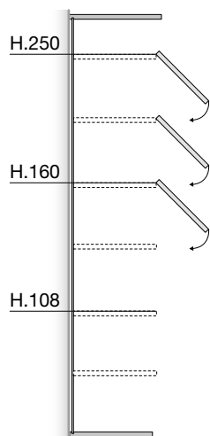
ANTA VASISTAS LIFT-UP DOOR
