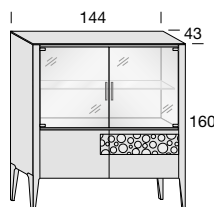
1 RIPIANO VETRO, 2 ANTE VETRO CON MANIGLIA, 2 ANTE LEGNO APERTURA PUSH PULL 1 GLASS SHELF, 2 GLASS DOORS WITH HANDLE, 2 WOODEN DOORS PUSH PULL OPENING SYSTEM
