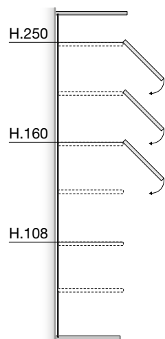
ANTA VASISTAS LIFT-UP DOOR
